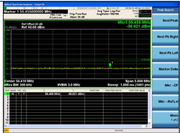
2th Harmonic
