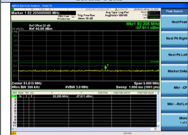
3th Harmonic
