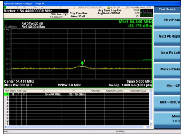
2th Harmonic
