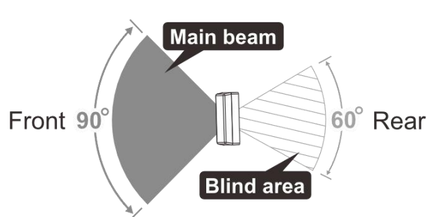
Indoor antenna
