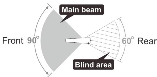
Outdoor antenna
