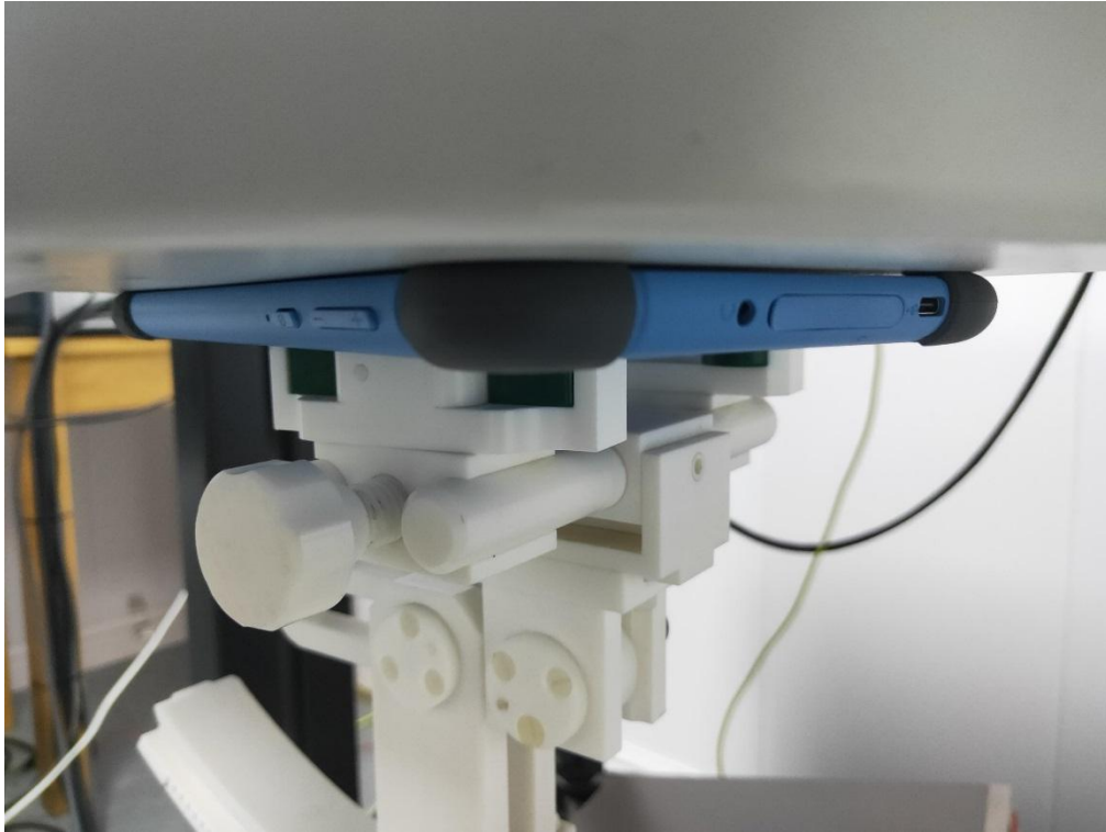
0mm body-worn Front Side Setup Photo
