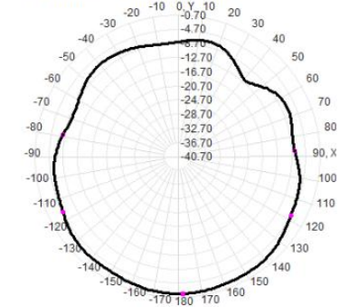
Total(H-XY), Max= -2.01dBi, CirD=10.10
