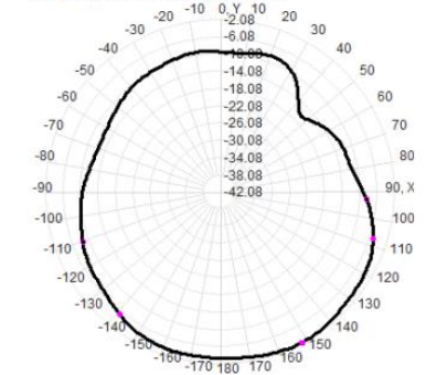
Total(H-XY), Max= -2.55dBi, CirD=13.99
