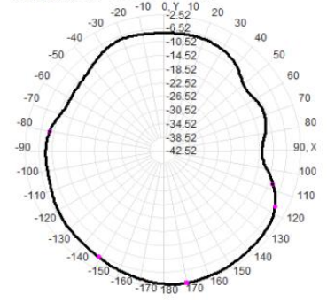
Total(H-XY), Max= -3.15dBi, CirD=10.94
