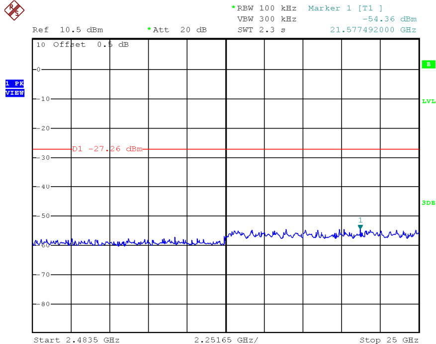
BT4 2Mbit, Lowest Channel, Plot B
