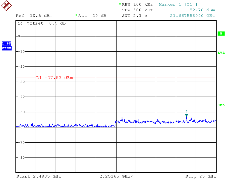
BT4 2Mbit, Middle Channel, Plot B
