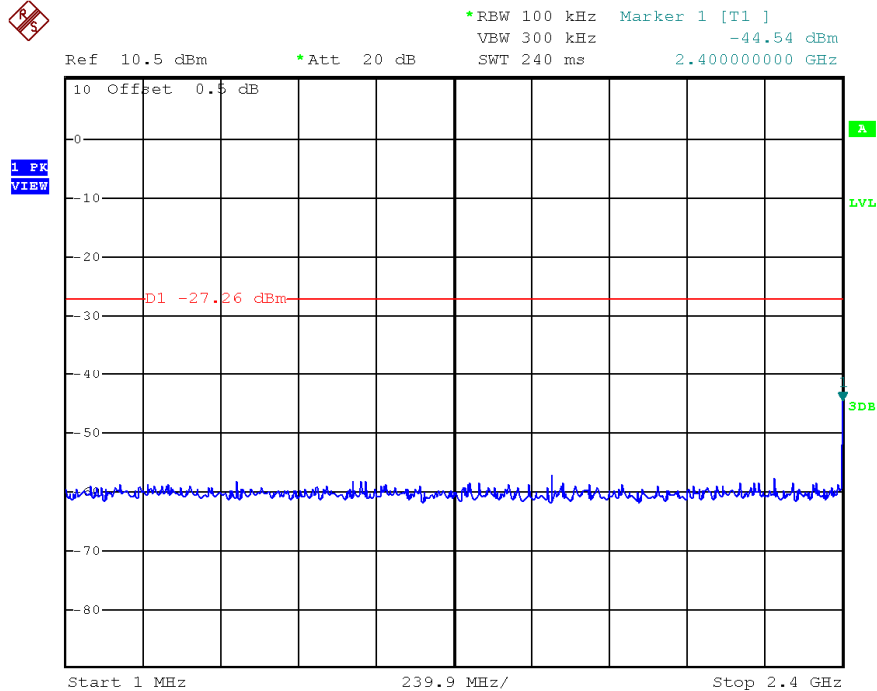
BT4 2Mbit, Lowest Channel, Plot A
