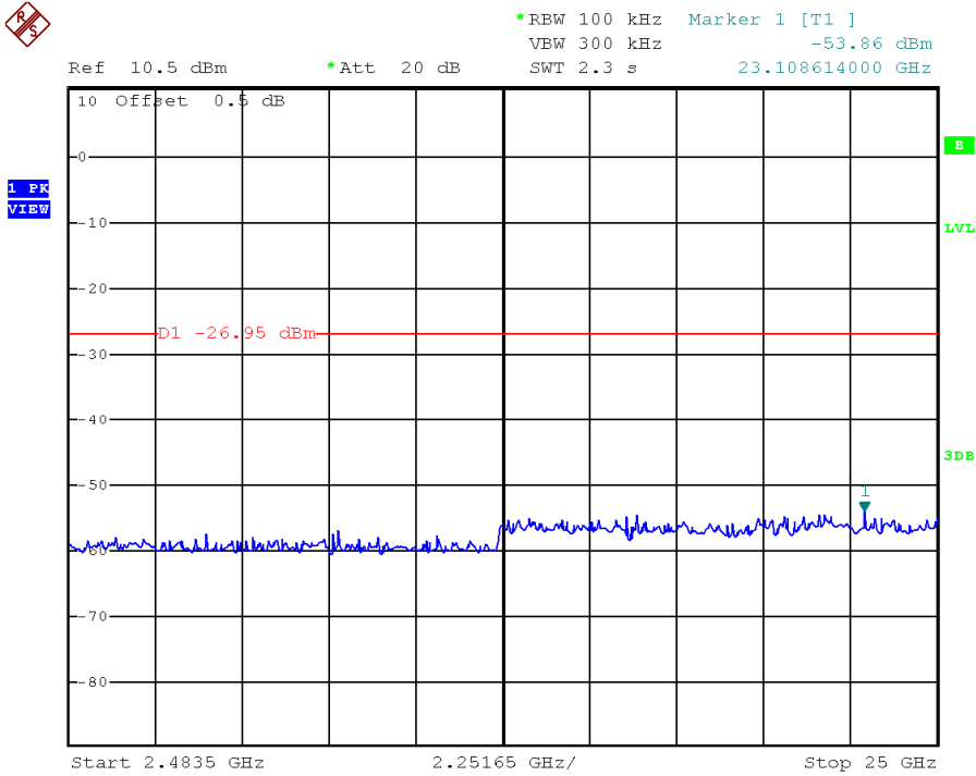
BT4 1Mbit, Middle Channel, Plot B
