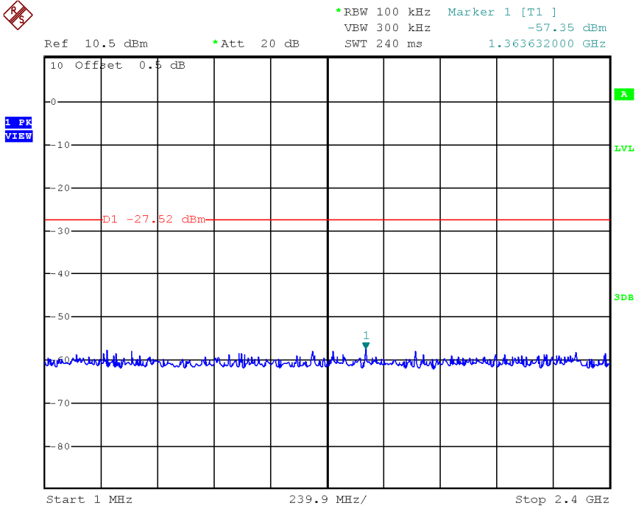
BT4 2Mbit, Middle Channel, Plot A
