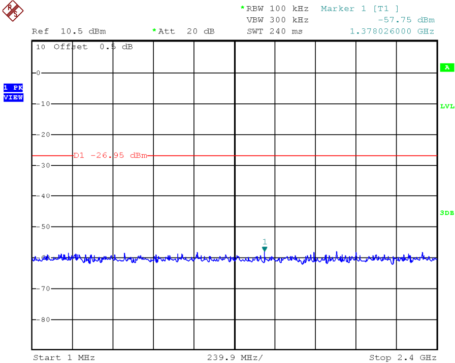
BT4 1Mbit, Middle Channel, Plot A
