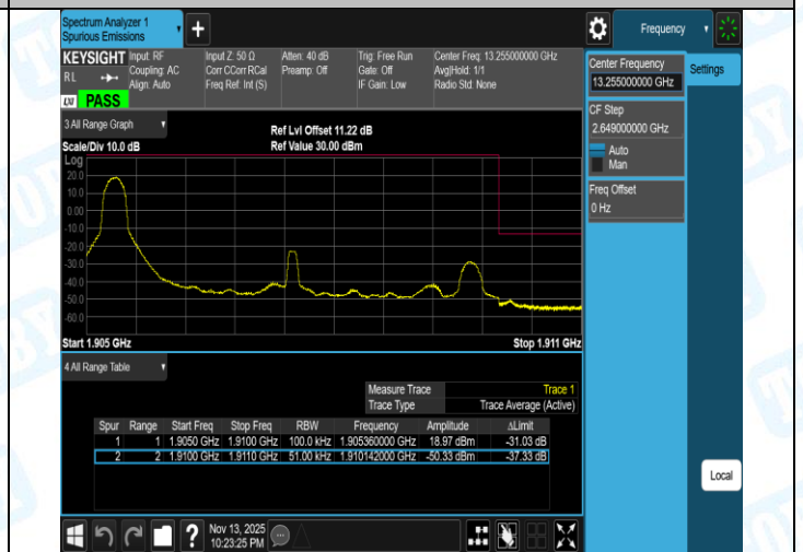
Band2-5MHz-16QAM-19175-25RB#0-PASS
