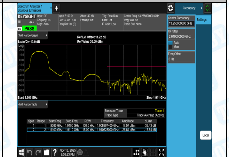
Band2-1.4MHz-16QAM-19193-6RB#0-PASS
