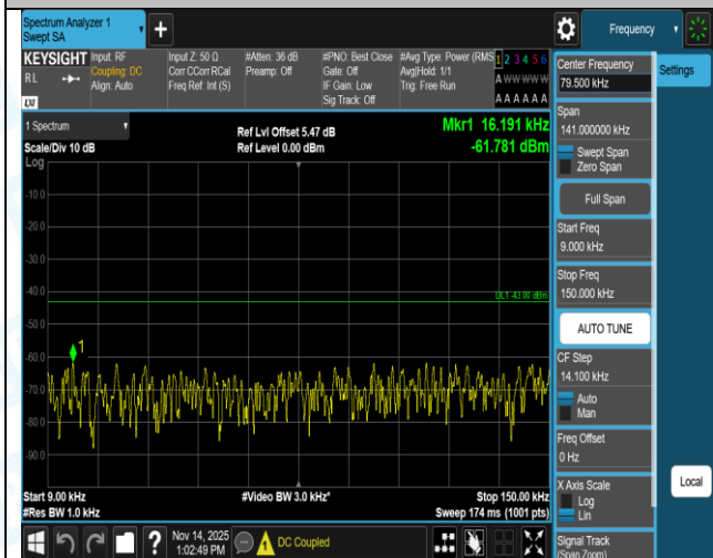
Band4-20MHz-QPSK-20300-100RB#0-30-1000-PASS
