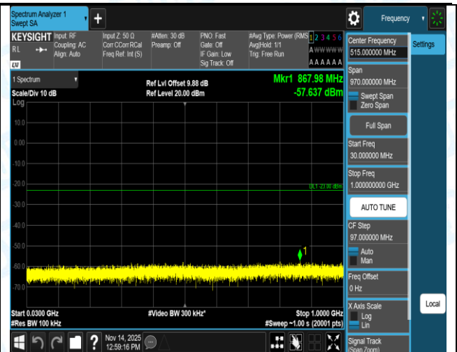
Band4-20MHz-QPSK-20300-1RB#99-3000-20000-PASS
