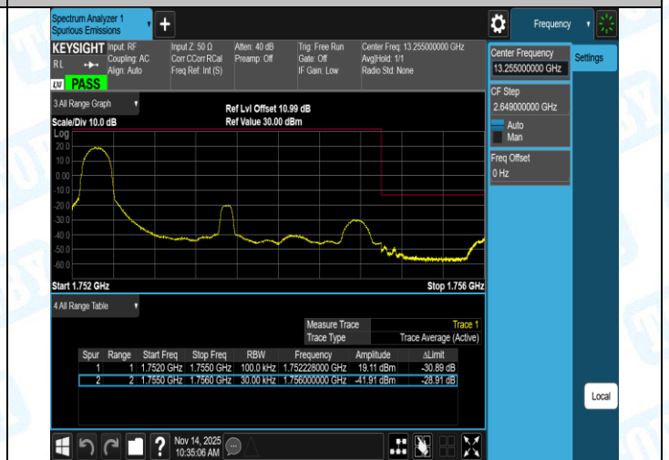
Band4-3MHz-QPSK-20385-15RB#0-PASS
