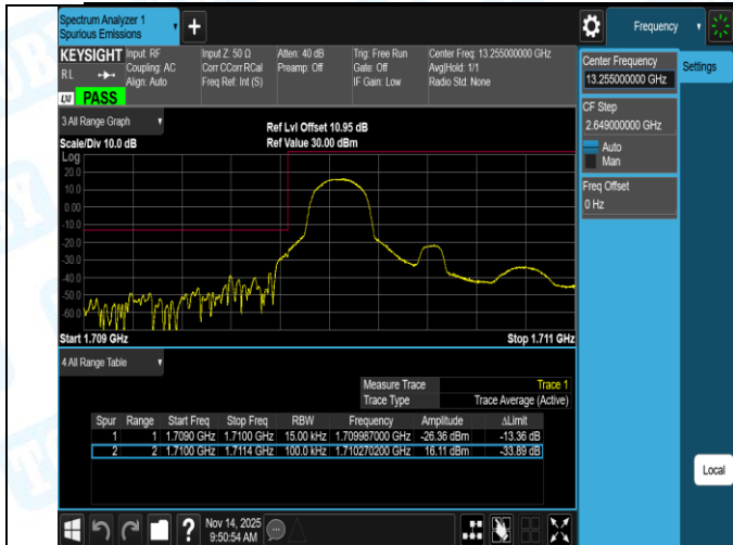
Band4-1.4MHz-16QAM-19957-6RB#0-PASS
