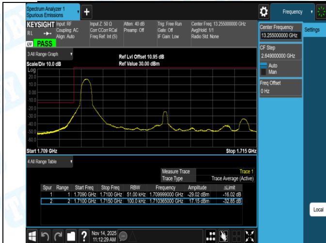
Band4-5MHz-16QAM-19975-25RB#0-PASS
