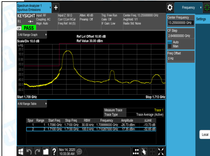
Band4-3MHz-QPSK-19965-15RB#0-PASS
