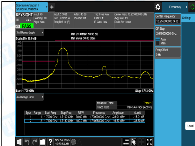
Band4-3MHz-16QAM-19965-15RB#0-PASS
