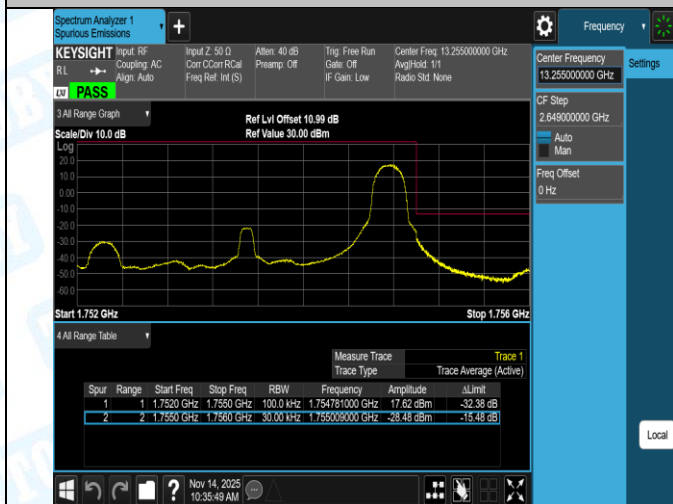
Band4-5MHz-QPSK-19975-1RB#0-PASS
