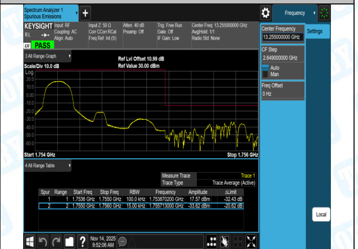
Band4-1.4MHz-16QAM-20393-6RB#0-PASS
