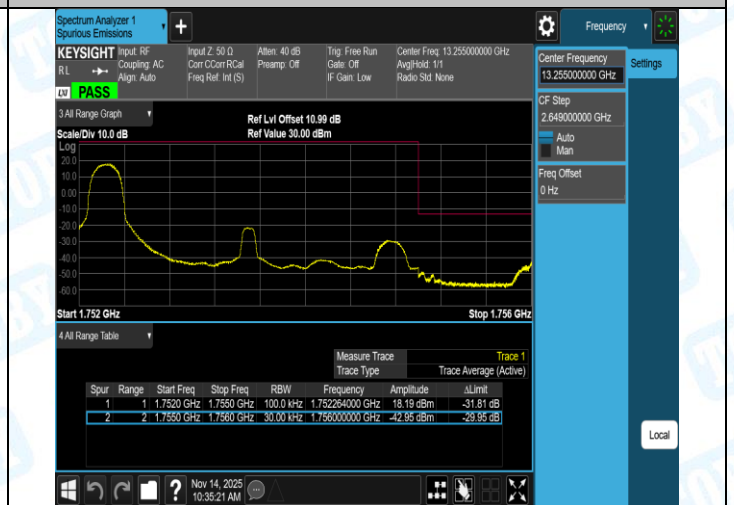
Band4-3MHz-16QAM-20385-15RB#0-PASS
