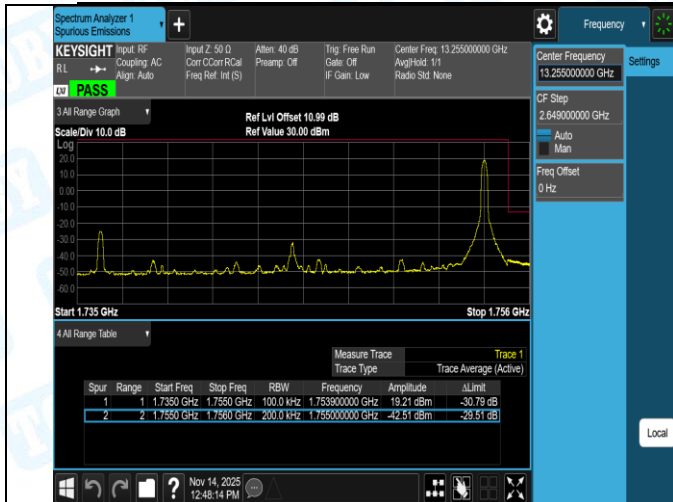
Band4-20MHz-16QAM-20050-1RB#0-PASS
