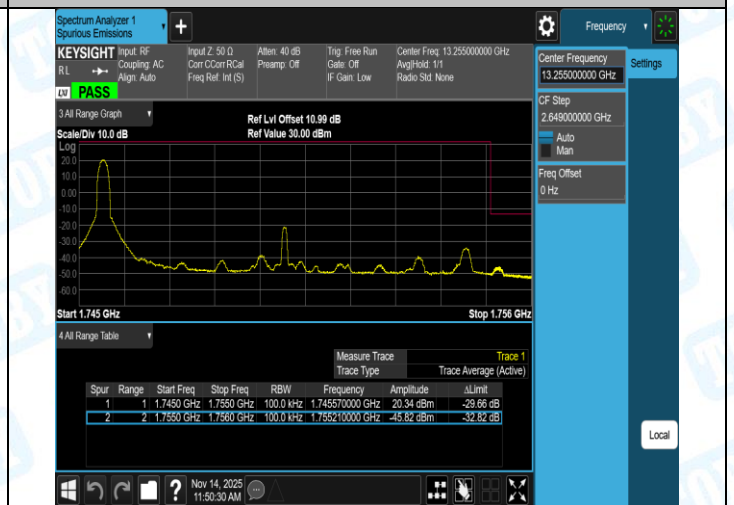
Band4-10MHz-QPSK-20350-50RB#0-PASS
