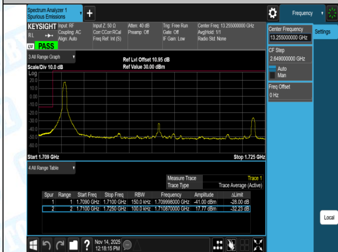
Band4-15MHz-QPSK-20025-75RB#0-PASS
