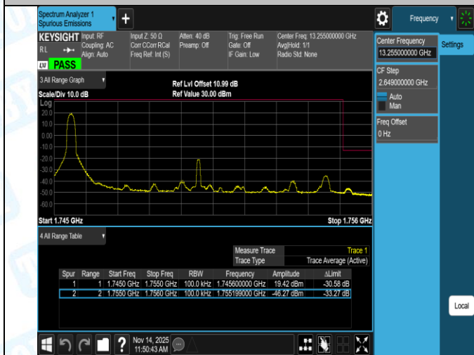
Band4-15MHz-QPSK-20025-1RB#0-PASS
