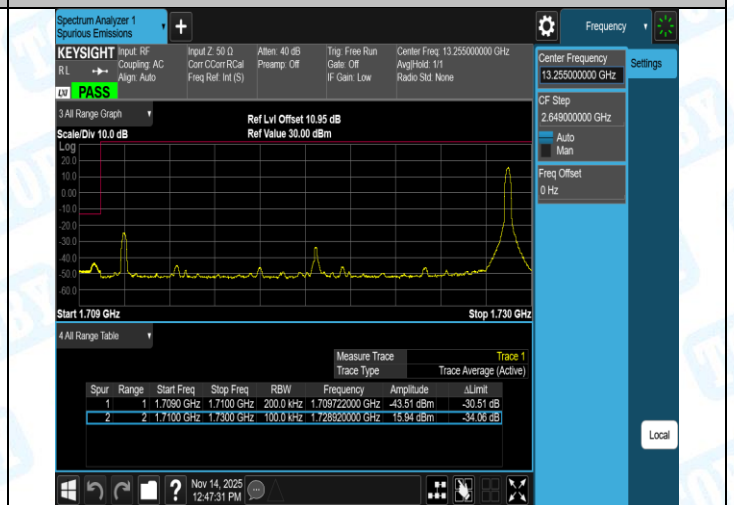
Band4-20MHz-16QAM-20300-1RB#99-PASS
