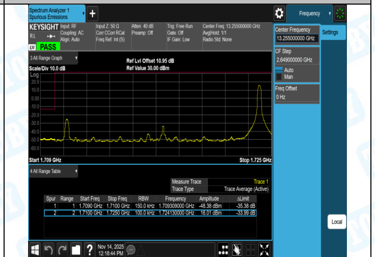
Band4-15MHz-QPSK-20325-1RB#0-PASS
