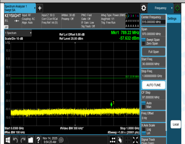
Band4-1.4MHz-16QAM-19957-1RB#0-3000~20000-PASS
