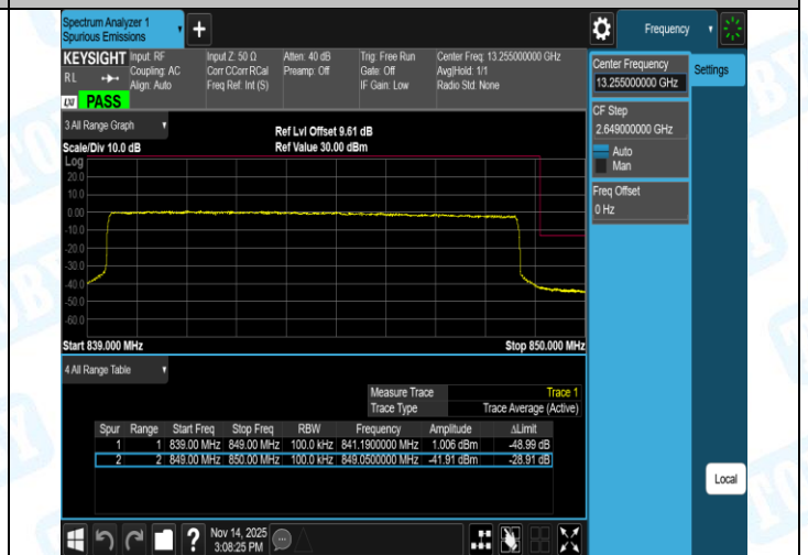
Band5-10MHz-16QAM-20450-1RB#49-PASS
