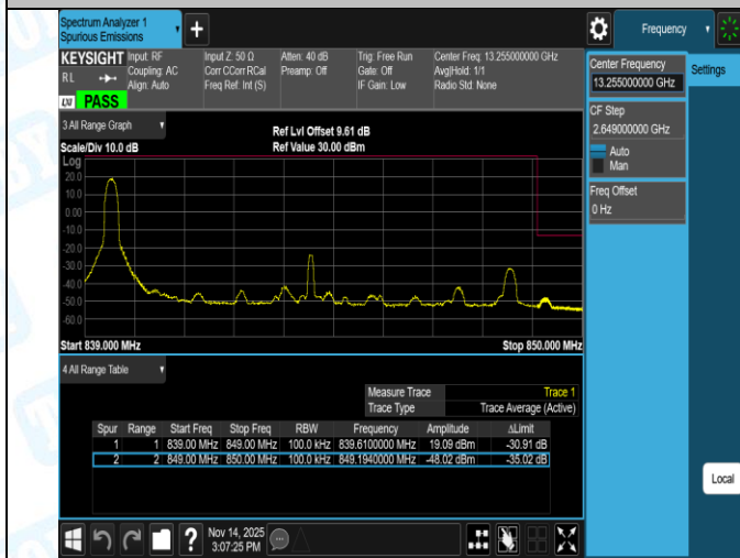
Band5-10MHz-16QAM-20600-1RB#0-PASS
