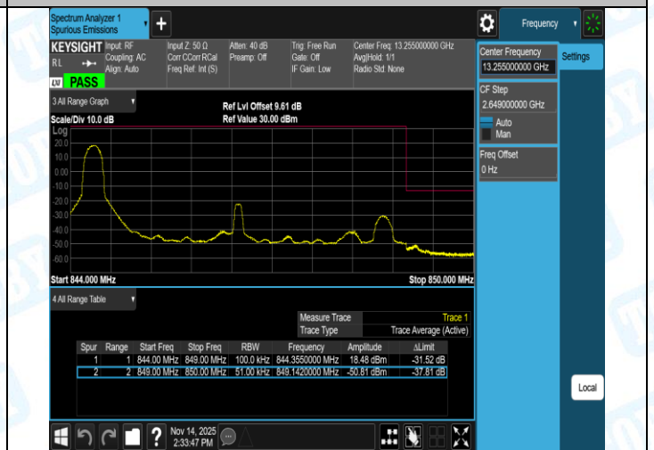
Band5-5MHz-16QAM-20625-25RB#0-PASS
