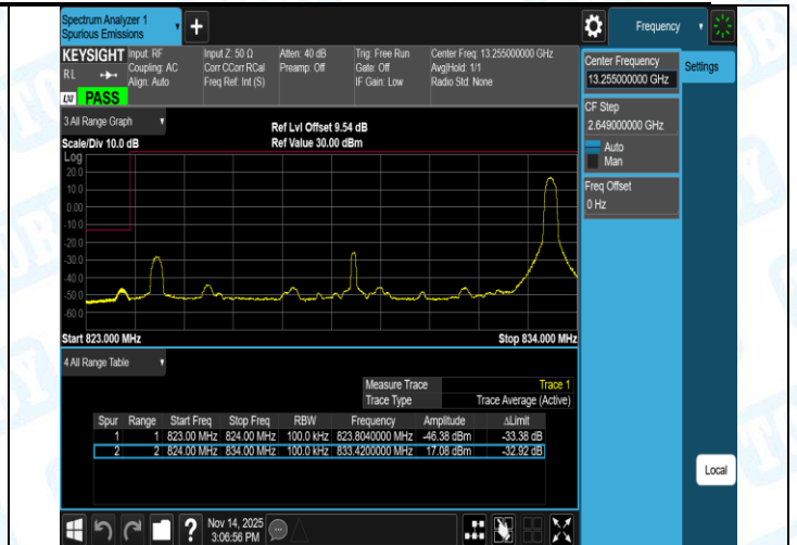
Band5-10MHz-16QAM-20600-1RB#49-PASS
