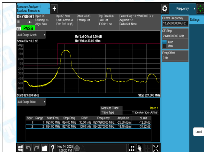
Band5-3MHz-16QAM-20415-15RB#0-PASS
