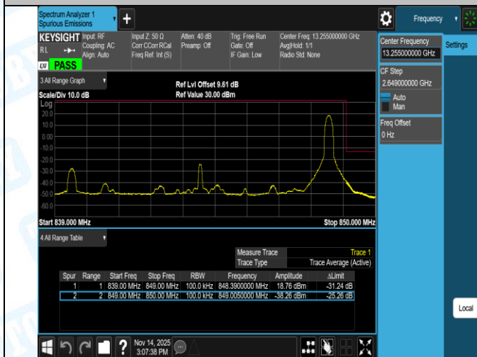
Band5-10MHz-16QAM-20450-1RB#0-PASS
