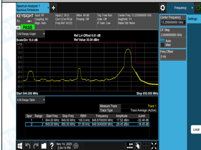
Band5-10MHz-QPSK-20450-1RB#0-PASS
