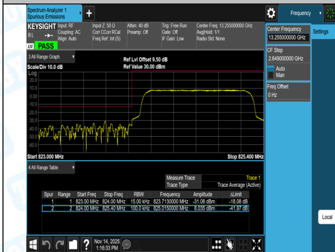
Band5-1.4MHz-16QAM-20643-1RB#5-PASS
