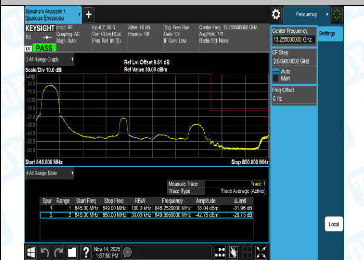
Band5-3MHz-16QAM-20635-15RB#0-PASS
