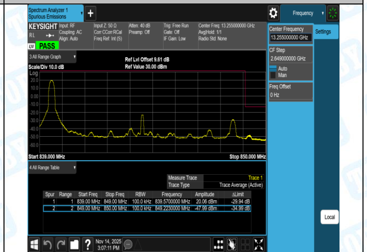
Band5-10MHz-QPSK-20600-50RB#0-PASS
