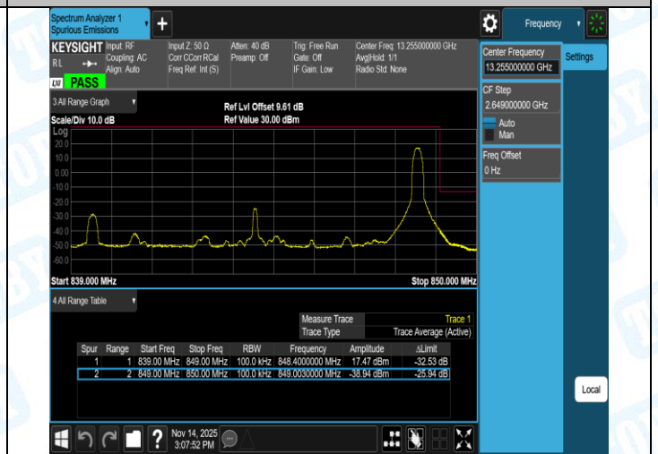
Band5-10MHz-16QAM-20600-1RB#49-PASS
