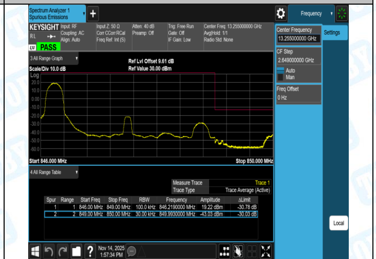
Band5-3MHz-QPSK-20635-15RB#0-PASS
