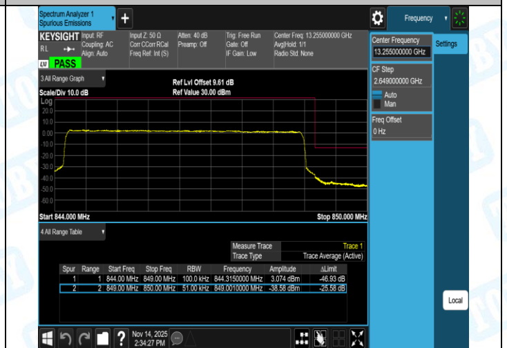
Band5-5MHz-16QAM-20425-1RB#24-PASS
