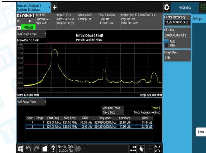
Band5-5MHz-16QAM-20425-25RB#0-PASS
