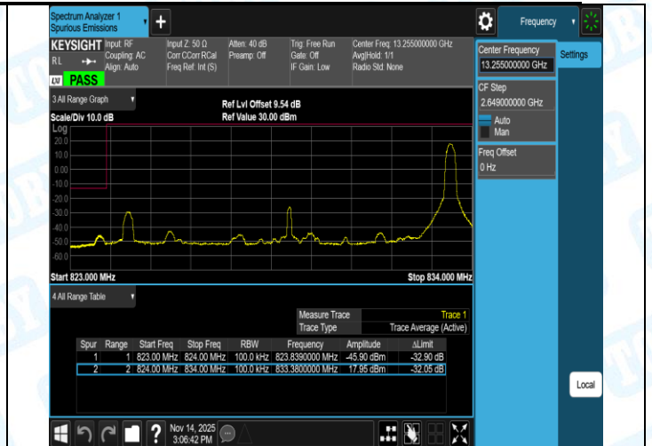
Band5-10MHz-QPSK-20600-1RB#0-PASS
