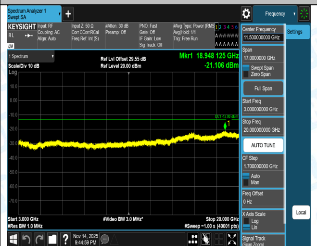
Band66-20MHz-QPSK-132072-1RB#0-0.15~30-PASS
