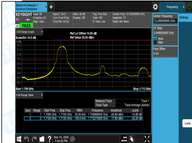
Band66-3MHz-16QAM-131987-15RB#0-PASS
