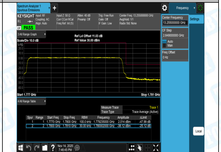
Band66-5MHz-QPSK-131997-1RB#24-PASS
