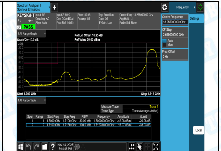
Band66-3MHz-16QAM-132657-1RB#0-PASS
