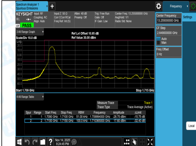
Band66-5MHz-16QAM-131997-25RB#0-PASS
