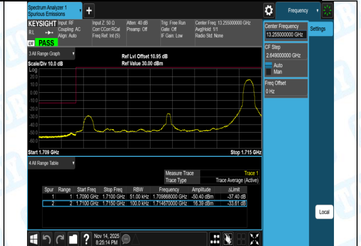
Band66-5MHz-16QAM-132647-1RB#0-PASS
