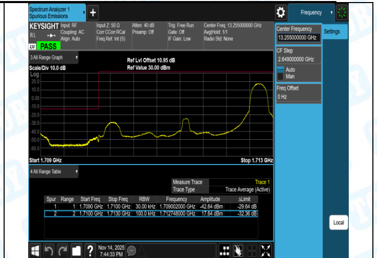
Band66-3MHz-QPSK-132657-1RB#0-PASS
