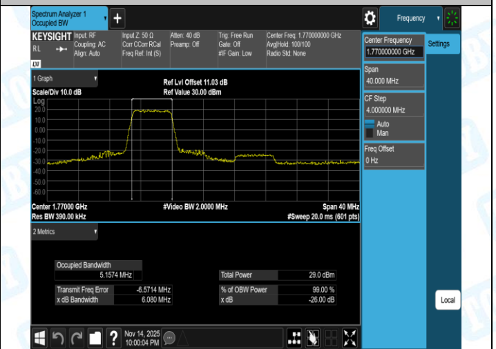
Band66-20MHz-16QAM-132572-27RB#0-PASS
