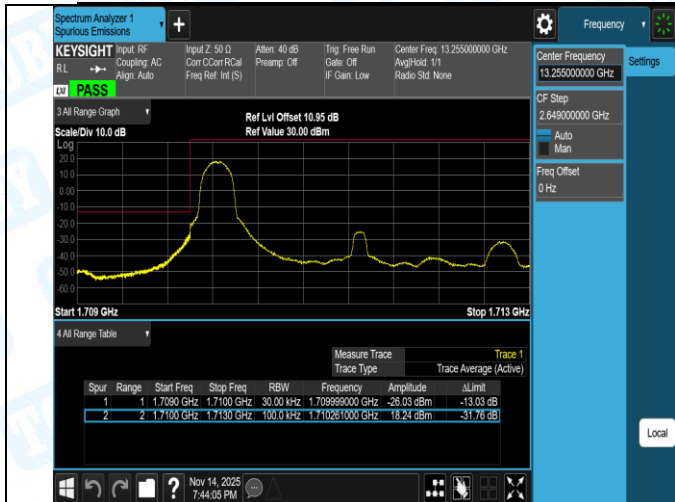
Band66-3MHz-QPSK-131987-15RB#0-PASS
