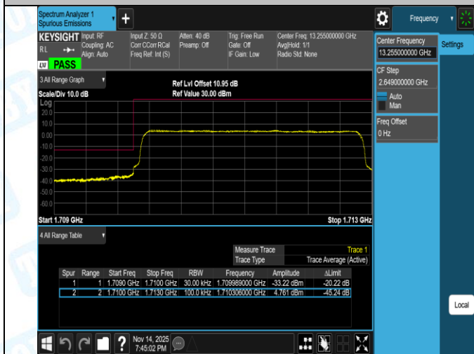
Band66-3MHz-QPSK-132657-1RB#14-PASS
