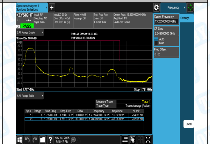
Band66-3MHz-16QAM-132657-15RB#0-PASS
