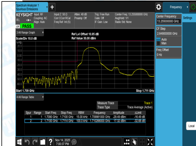
Band66-1.4MHz-16QAM-131979-6RB#0-PASS
