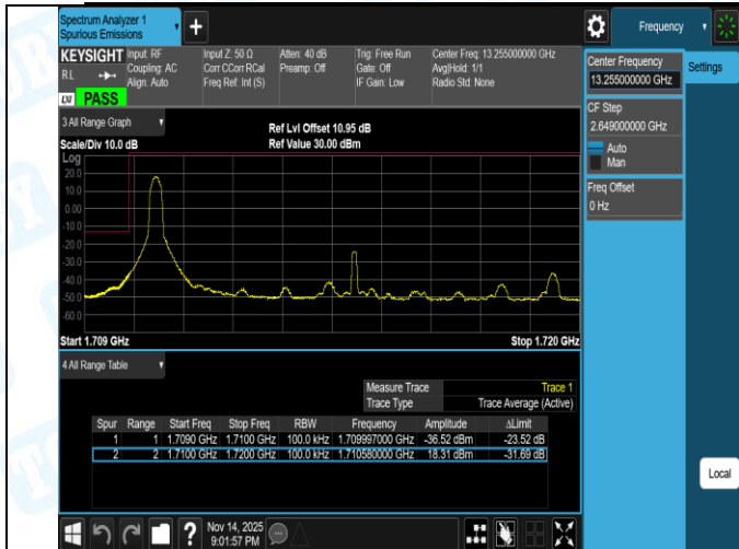
Band66-10MHz-QPSK-132022-50RB#0-PASS
