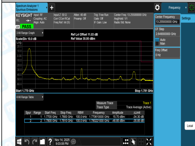
Band66-15MHz-QPSK-132047-1RB#0-PASS
