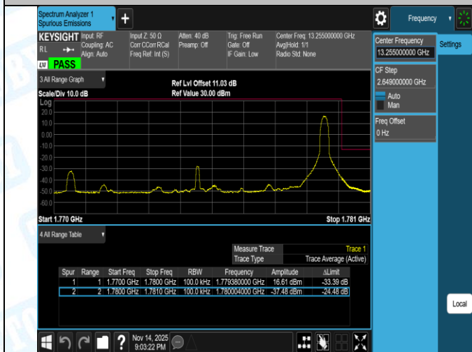
Band66-10MHz-16QAM-132022-1RB#0-PASS
