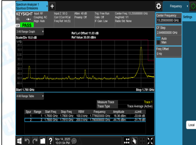
Band66-20MHz-16QAM-132072-1RB#0-PASS
