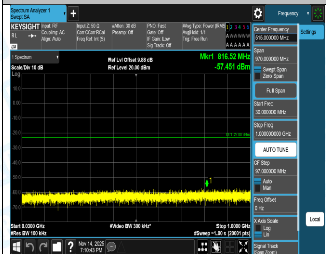
Band66-1.4MHz-QPSK-132322-1RB#5-3000-20000-PASS
