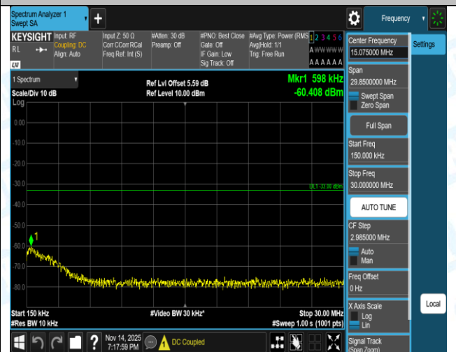
Band66-1.4MHz-QPSK-132665-6RB#0-1000~3000-PASS
