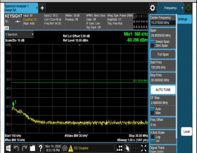
Band66-5MHz-QPSK-131997-25RB#0-1000~3000-PASS
