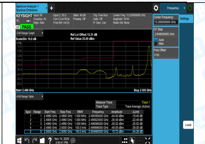
Band7-5MHz-16QAM-21425-1RB#0-PASS
