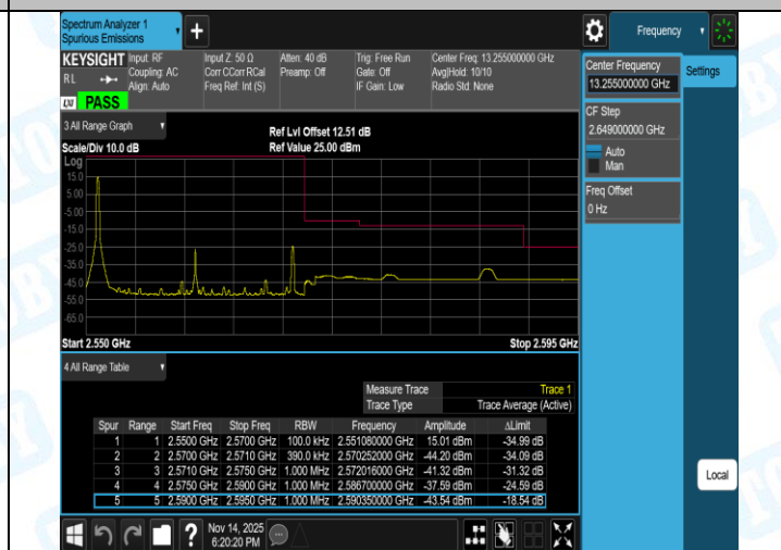
Band7-20MHz-QPSK-21350-100RB#0-PASS
