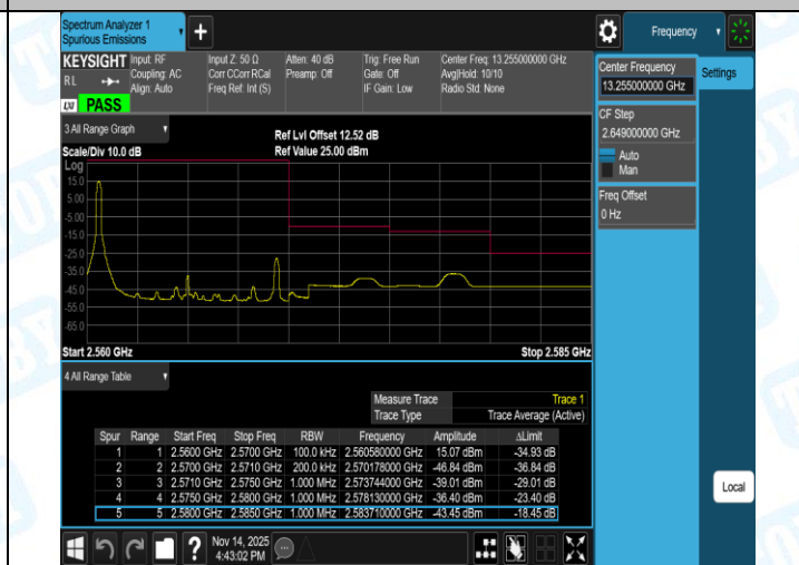
Band7-10MHz-QPSK-21400-50RB#0-PASS
