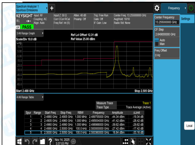
Band7-5MHz-16QAM-20775-25RB#0-PASS
