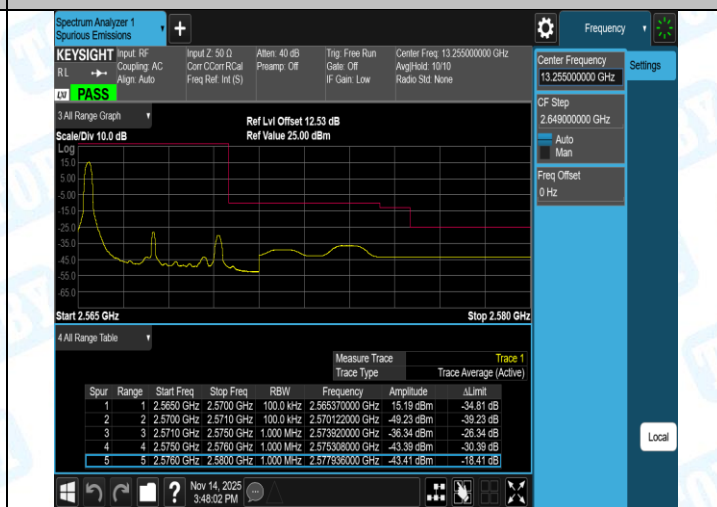
Band7-5MHz-16QAM-21425-25RB#0-PASS
