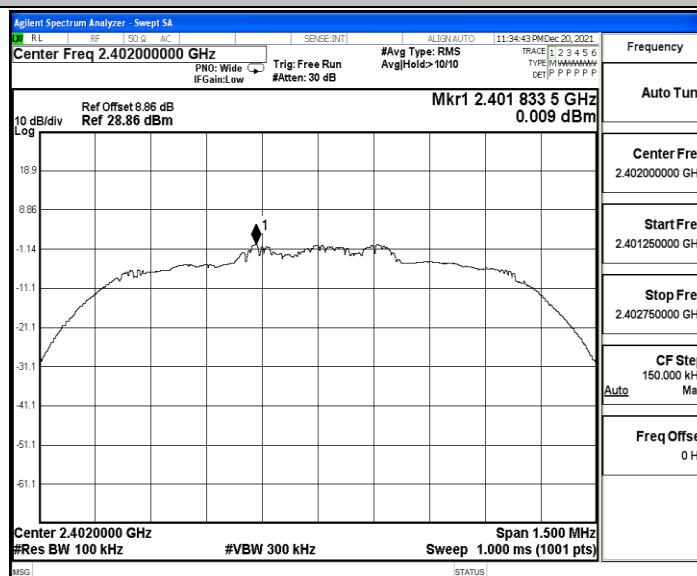
2DH5_BT ANT_2402_0~Reference
