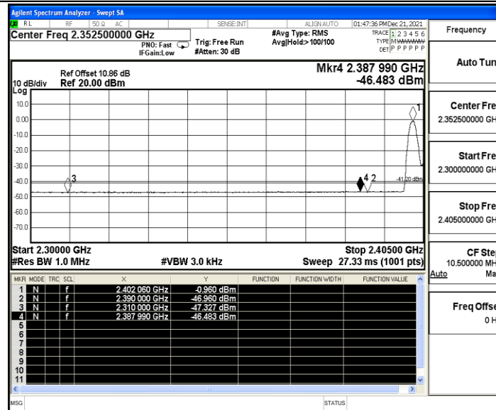
BLE_1M_BT ANT_Low_2402_Peak
