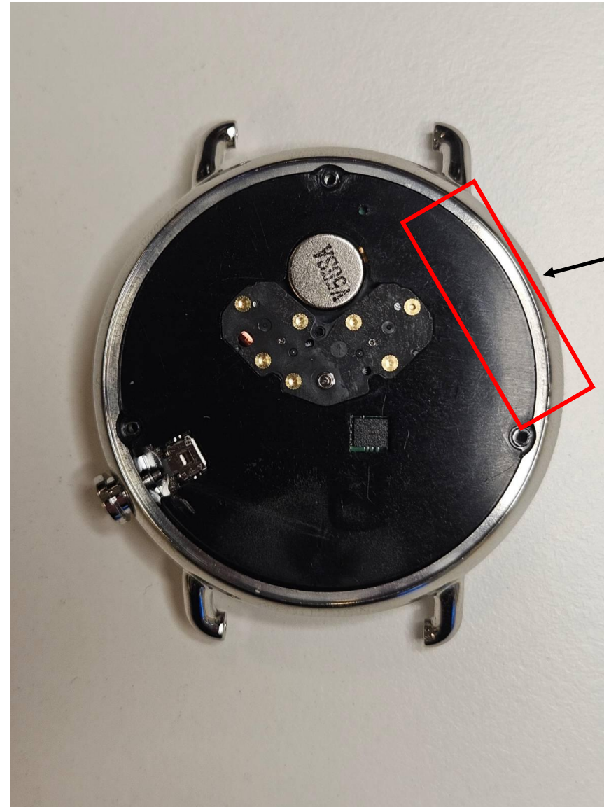
Antenna frame assembled
