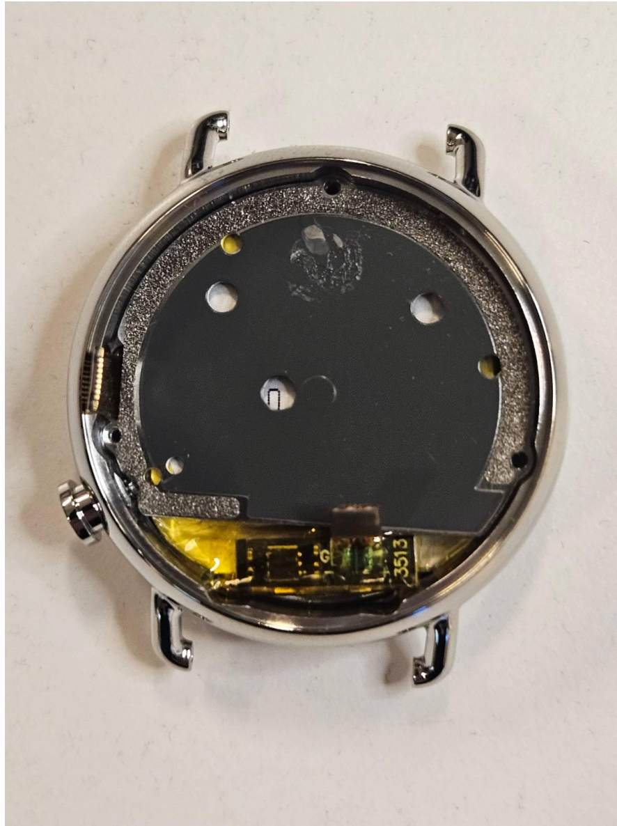
Support plate assembled
