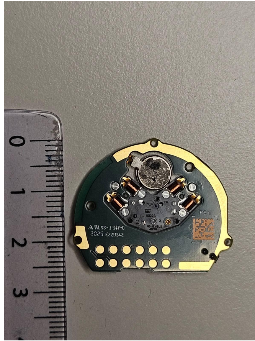
Main PCB back
