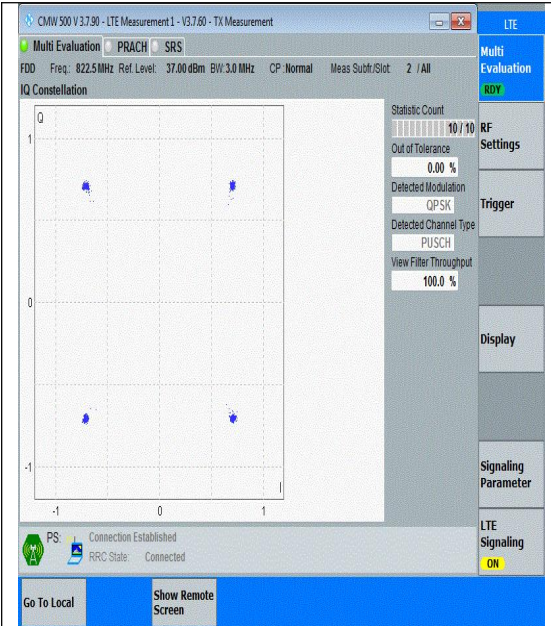
Band26(814-824)-3MHz-QPSK-26775-15RB#0-P
