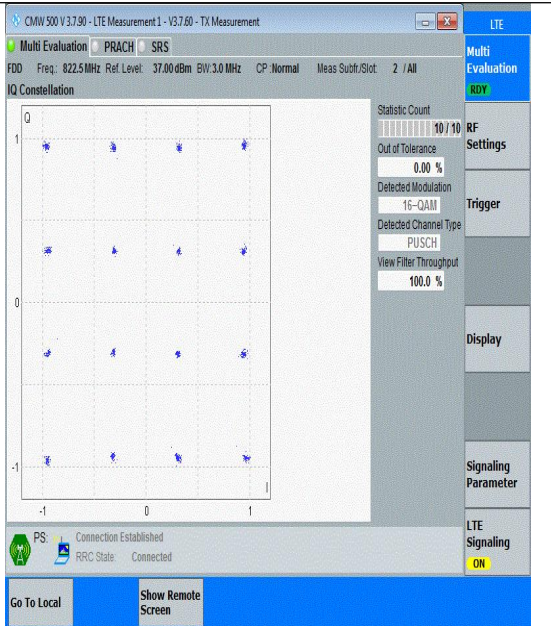
Band26(814-824)-3MHz-16QAM-26775-15RB#0-P
