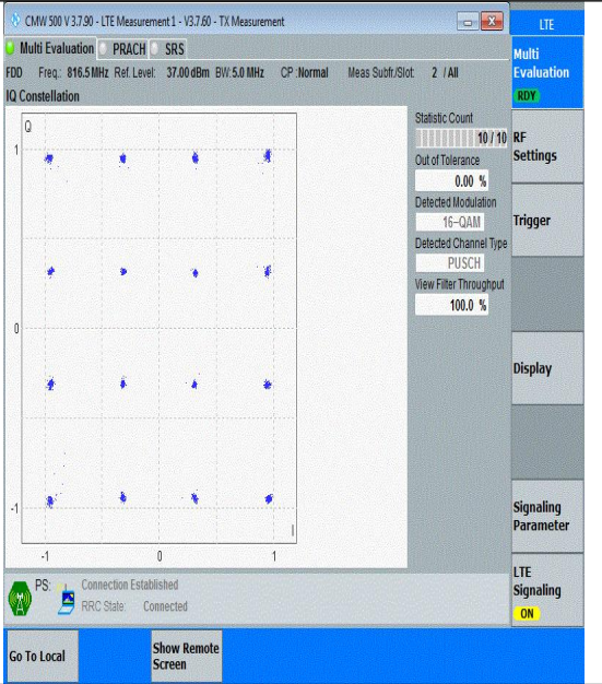
Band26(814-824)-5MHz-16QAM-26715-25RB#0-P
