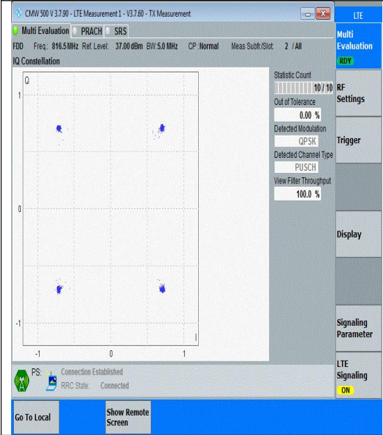
Band26(814-824)-5MHz-QPSK-26715-25RB#0-P
