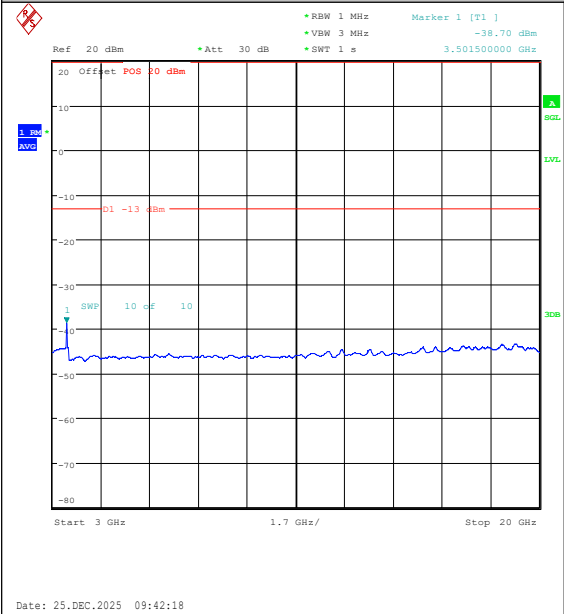
Band4-20MHz-QPSK-20300-1RB#99-3000~2000 0-PASS
