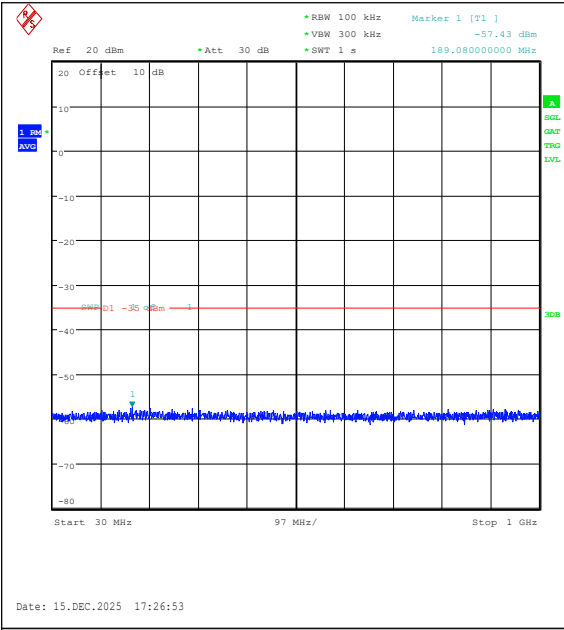
Band41(2535-2655)-5MHz-16QAM-40065-1RB#2 4-30~1000-PASS
