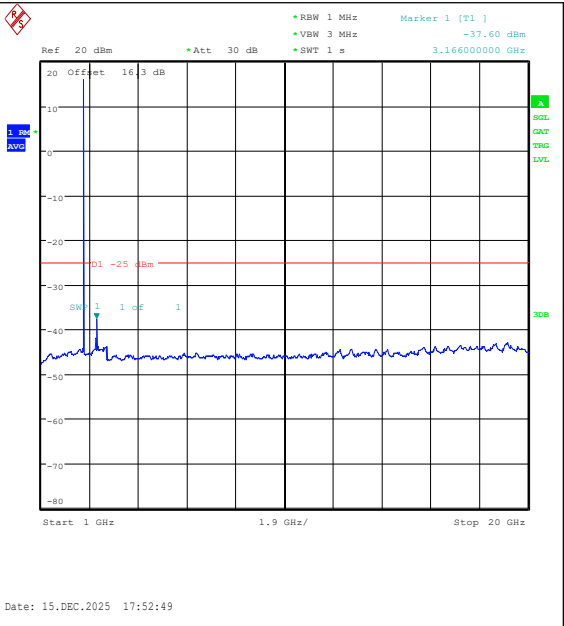
Band41(2535-2655)-5MHz-QPSK-41215-1RB#0-1000~20000-PASS
