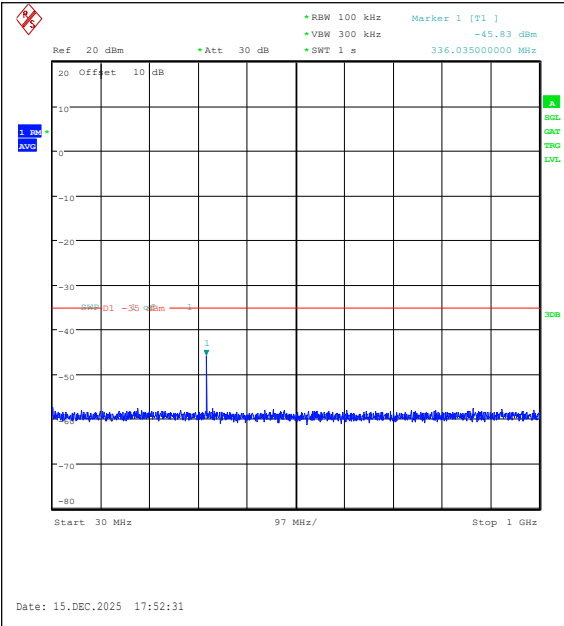
Band41(2535-2655)-5MHz-QPSK-41215-1RB#0-30~1000-PASS
