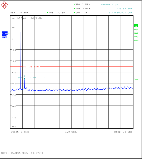
Band41(2535-2655)-5MHz-16QAM-40065-1RB#24 -1000~20000-PASS
