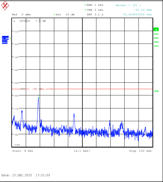
Band41(2535-2655)-5MHz-16QAM-40065-25RB#0 -0.009~0.15-PASS
