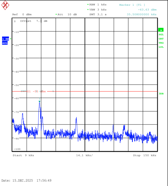
Band41(2535-2655)-5MHz-QPSK-41215-1RB#24-0.009~0.15-PASS
