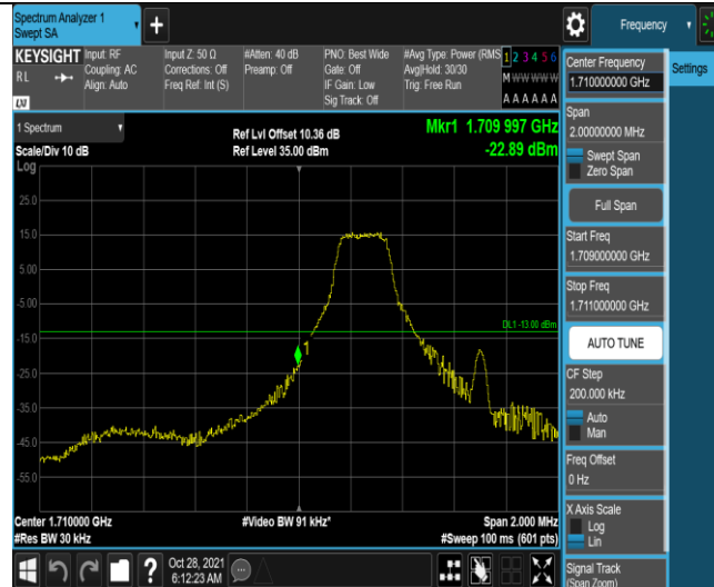
Band4-1.4MHz-16QAM-19957-1RB#5
