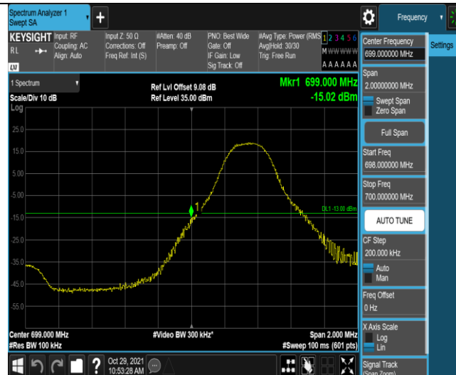
Band12-5MHz-16QAM-23035-1RB#24
