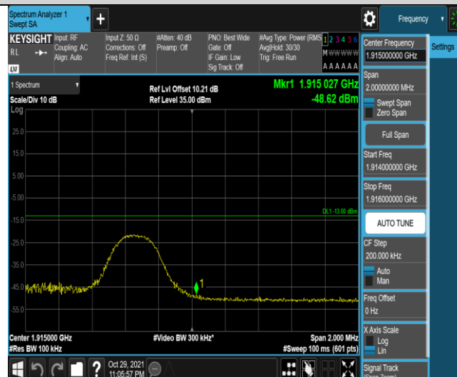
Band25-5MHz-16QAM-26665-1RB#24
