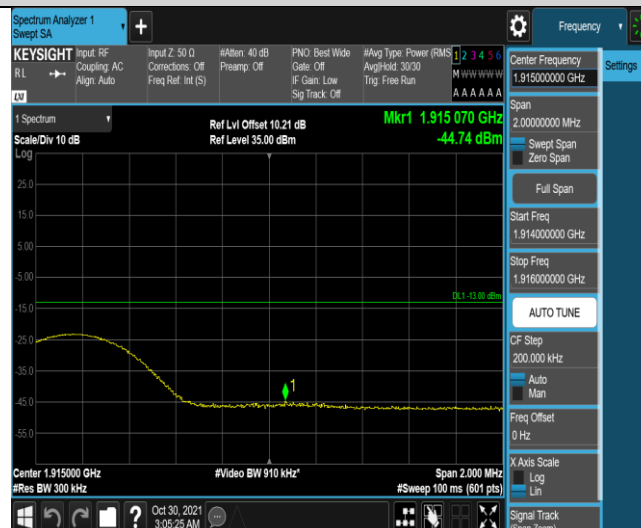
Band25-15MHz-QPSK-26615-1RB#74
