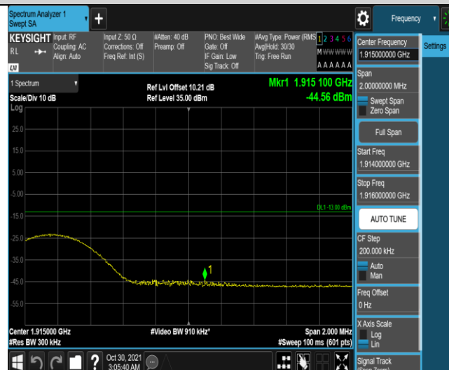
Band25-15MHz-16QAM-26615-1RB#74
