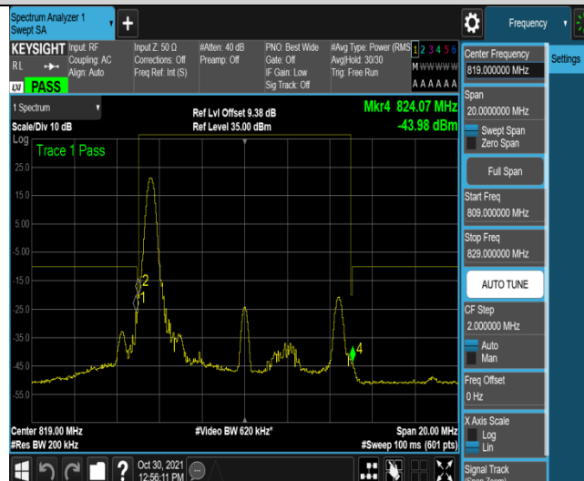
Band26-10MHz-16QAM-26740-1RB#49
