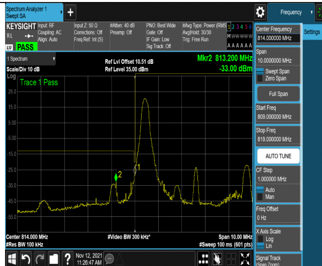
Band26-5MHz-16QAM-26715-1RB#24
