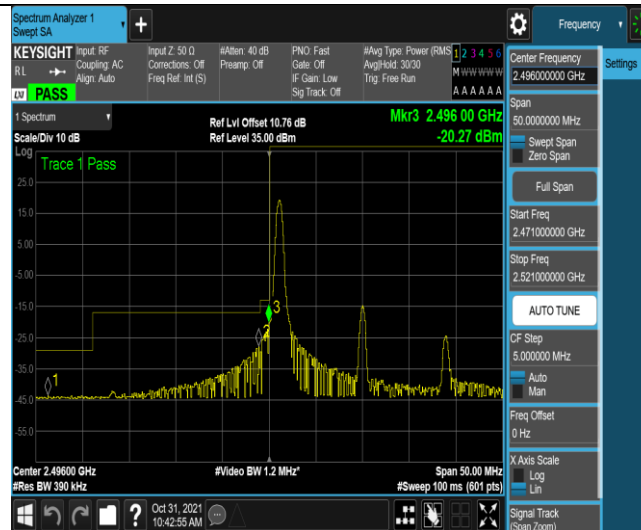
Band41-20MHz-16QAM-39750-1RB#99
