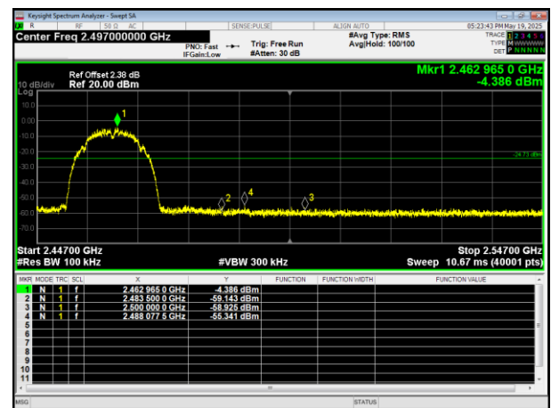
Highest Emission
