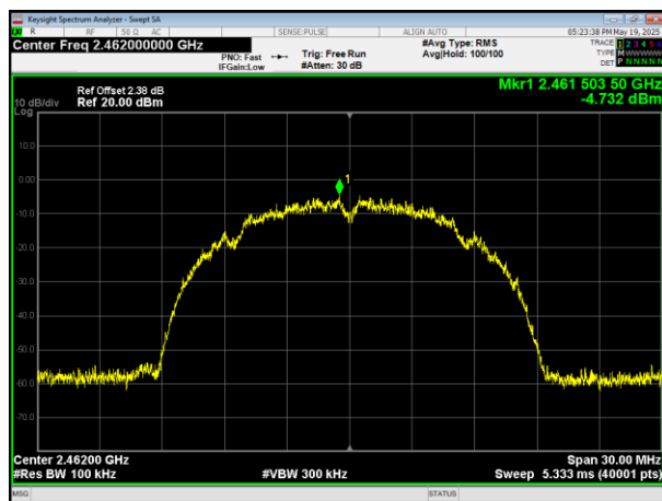
Highest Ref
