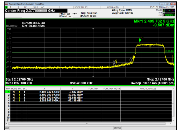
Lowest Emission
