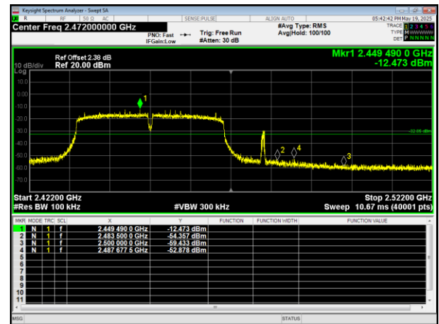
Highest Emission
