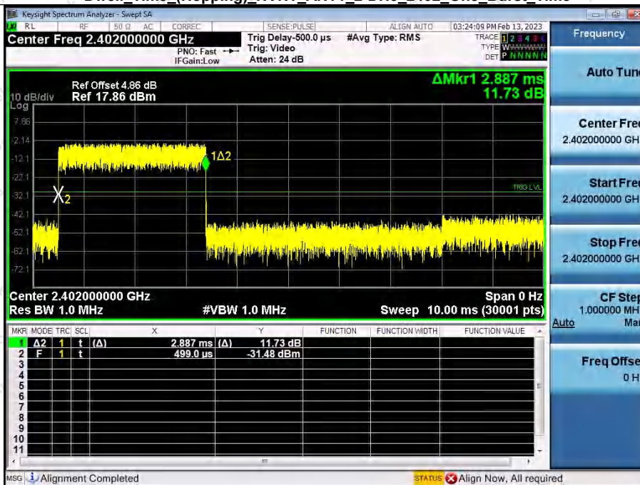
Dwell Time (Hopping) NVNT ANT1 2-DH5 2402 One Burst Time
