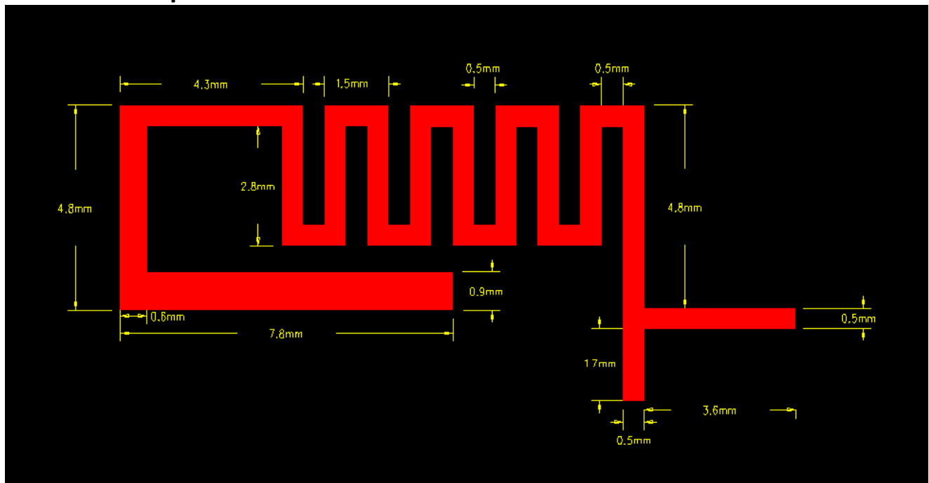
Antenna shape
