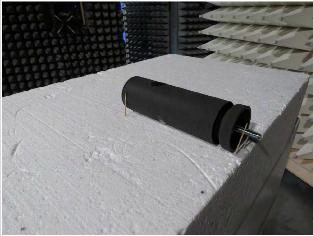
Setup EUT alignment horizontal
