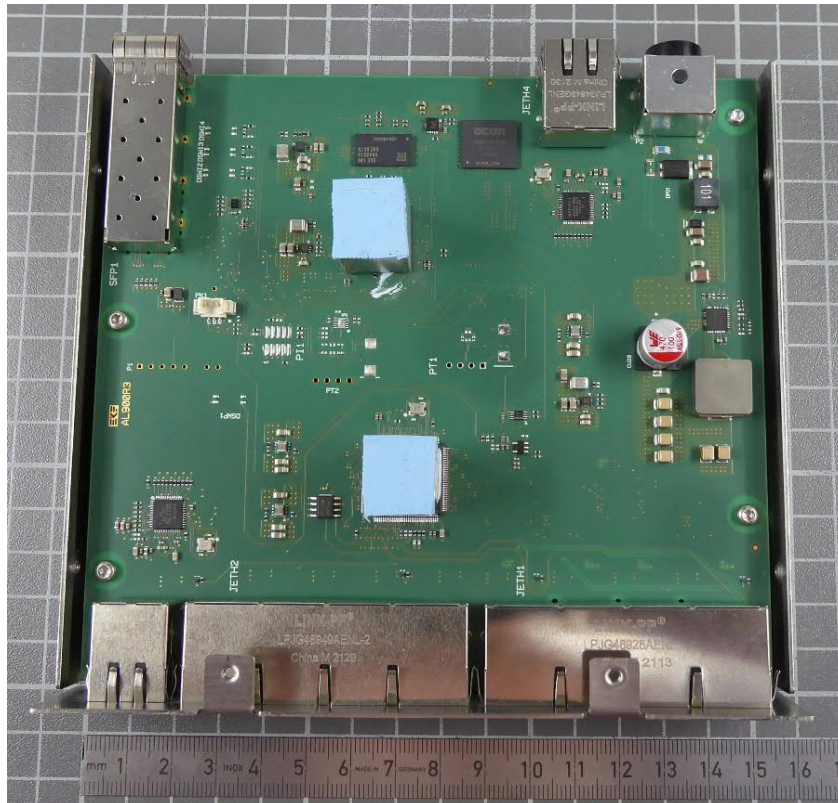
Photo 1: EUT/Enclosure open top view
