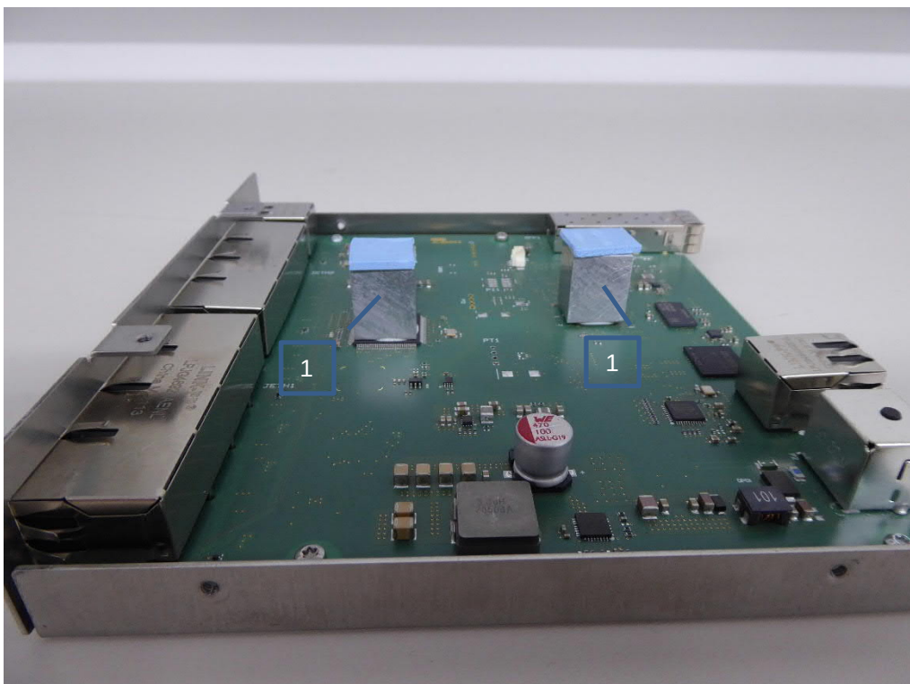
Photo 2: EUT/Enclosure open oblique view from above Note 1: Heatsink with Thermo pad
