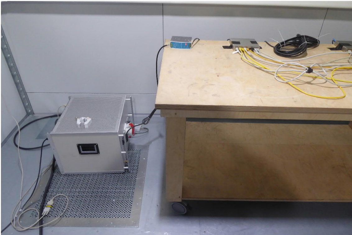
Test setup 2: Conducted Emission/Test point AC
