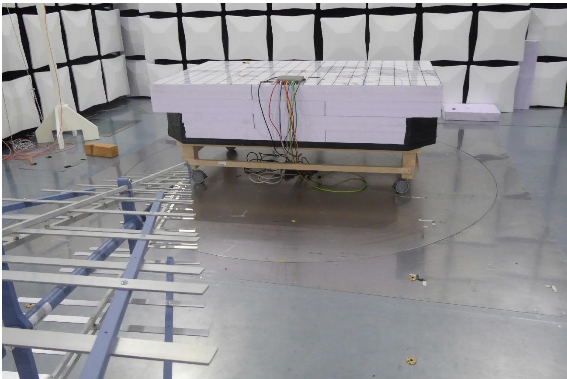
Test setup 4: Radiated Emission/30 MHz – 1 GHz
