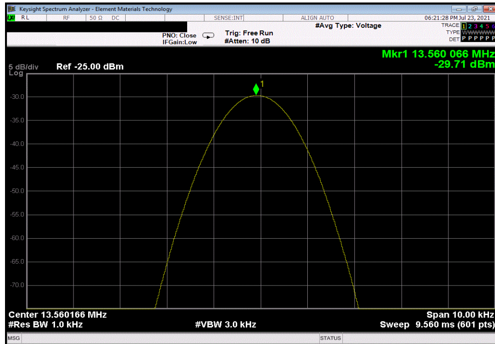
CrossSwitch Radio - Antenna 2, Extreme Temperature 0°C, Mid Channel, 13.56 MHz
