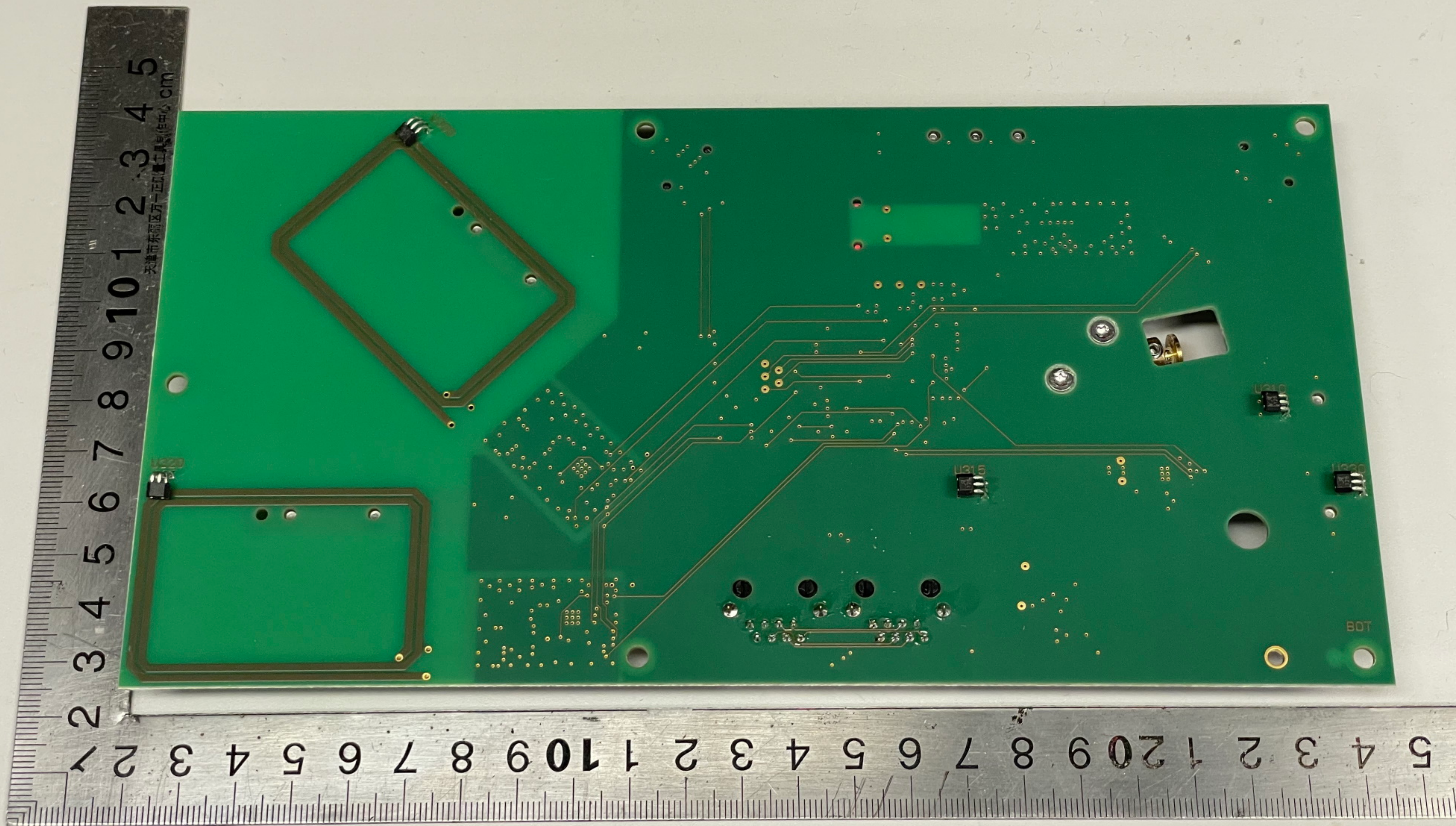
RFID SwitchController roundabout PCB
