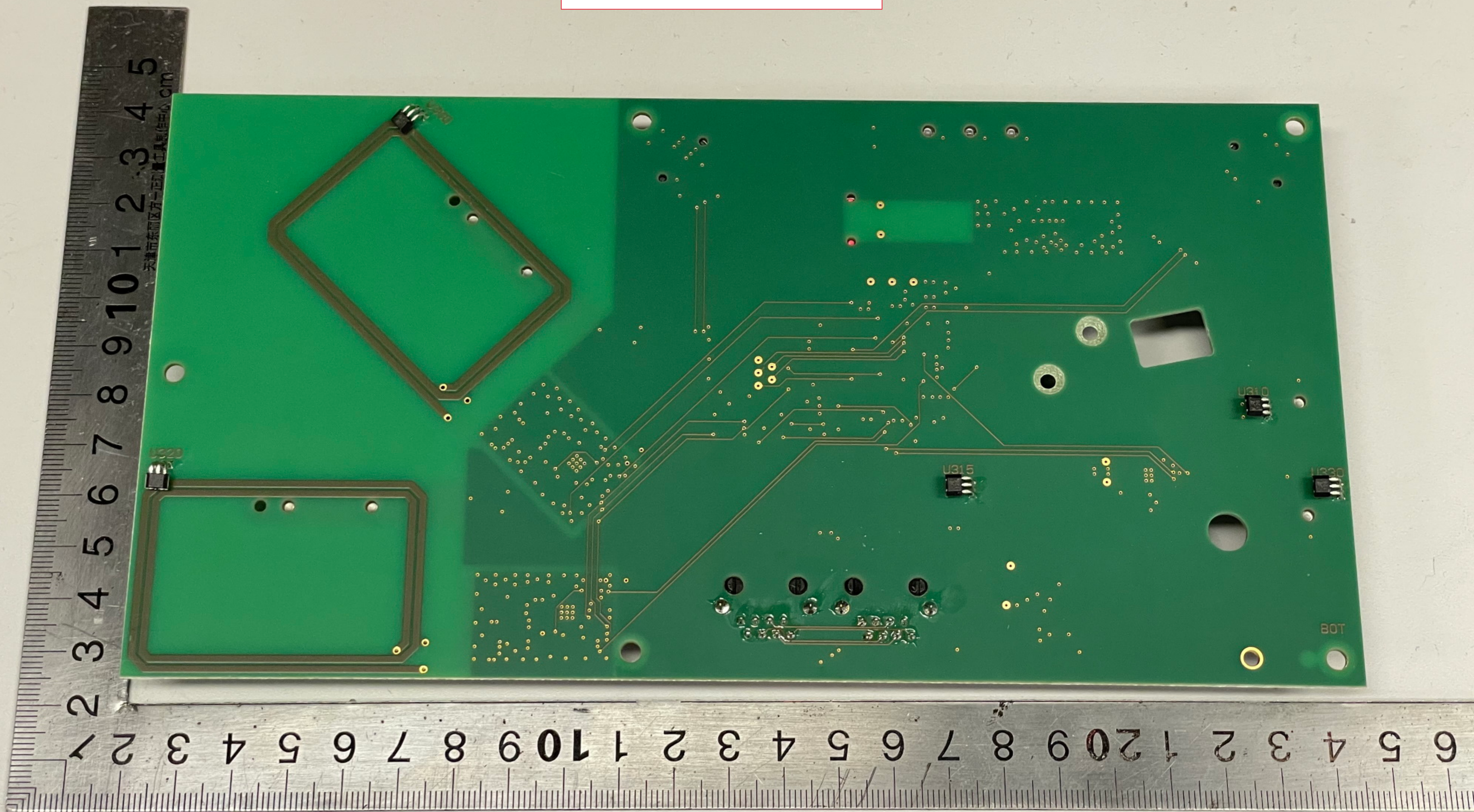
RFID SwitchController roundabout PCB
