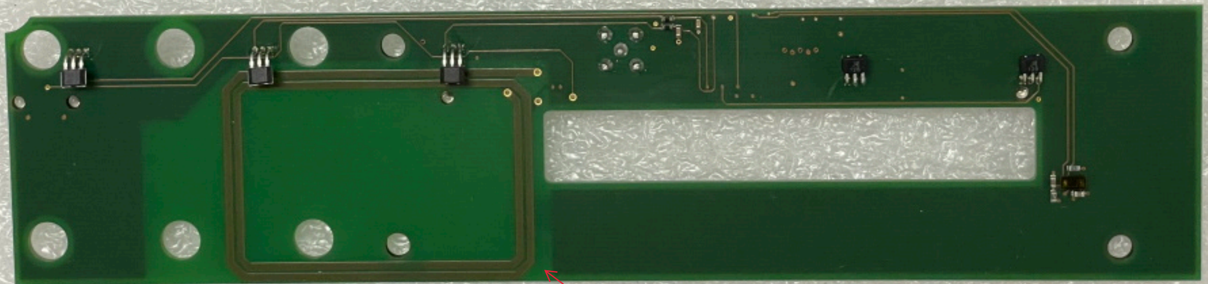
Weighing IO 20012202 Inductive Loop Antenna 51mm x 35mm
