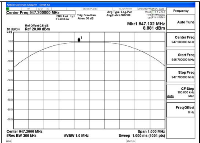
Channel 17 / 947.2 MHz
