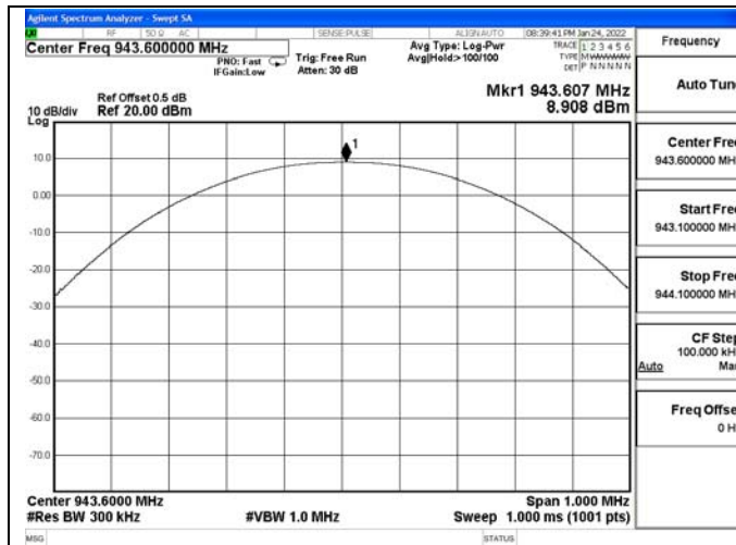
Channel 7 / 943.6 MHz
