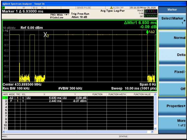
(Time per burst: 6.930ms*1pcs)
