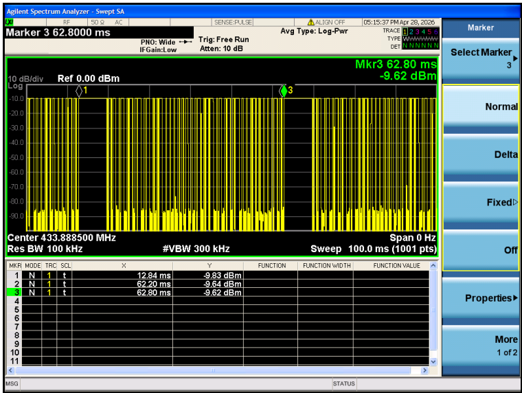
(Transmit cycle 49.96ms)
