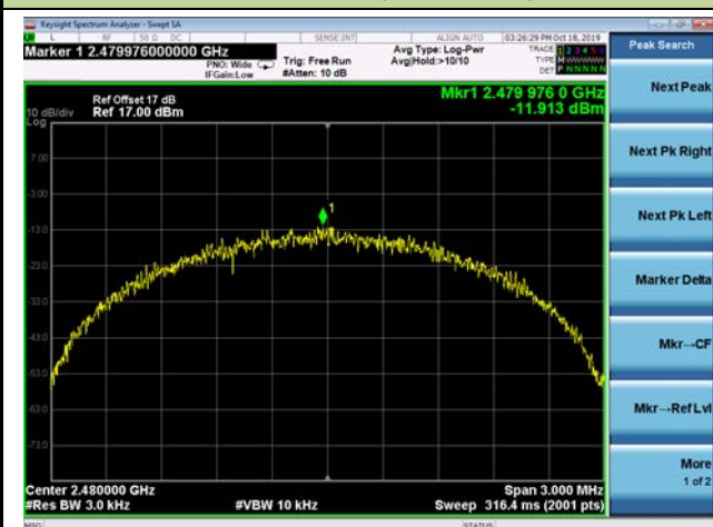
Channel 39 (2480MHz)
