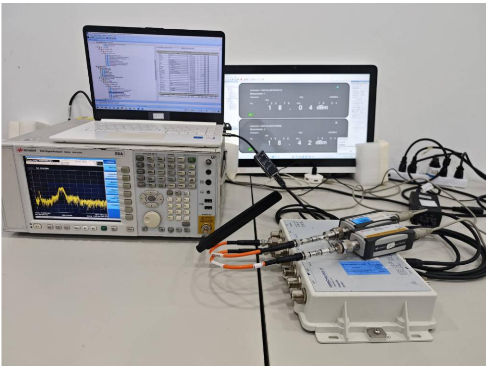
Description: Conducted Emission Test Setup – 2.4G
