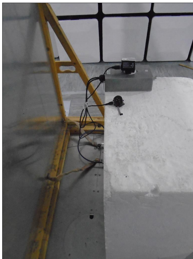
Figure 69 - AC Line Conducted Emissions
