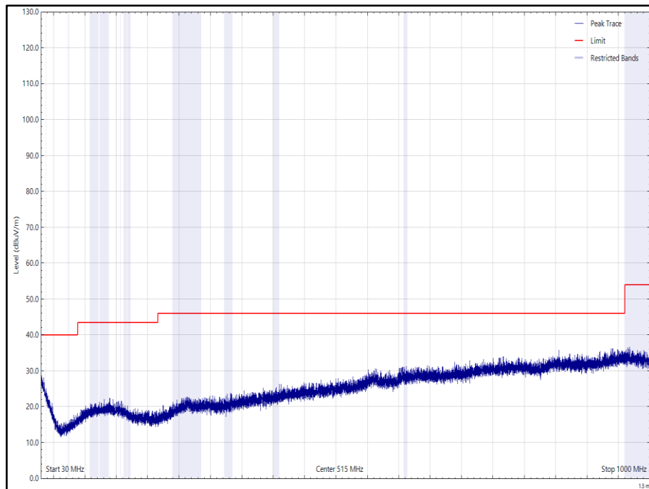
Figure 42 - CH39 (2480 MHz), LE1M, Orientation: Y, 30 MHz to 1 GHz, Horizontal (Peak)
