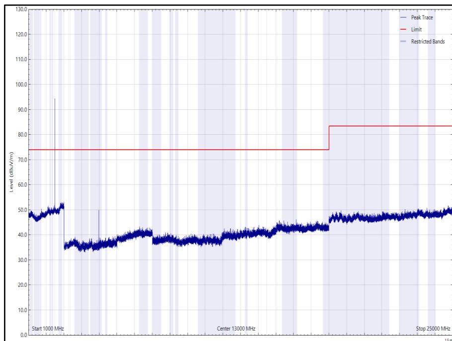
Figure 43 - CH39 (2480 MHz), LE1M, Orientation: Y, 1 GHz to 25 GHz, Horizontal (Peak)
