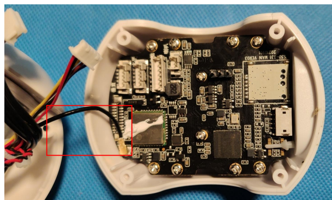
Antenna port
