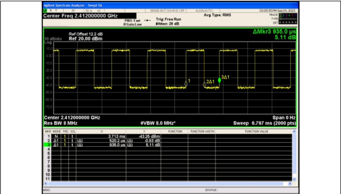
IEEE 802.11g 20MHz Channel 1
