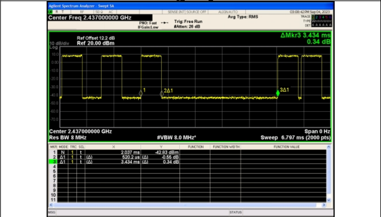
IEEE 802.11g 20MHz Channel 6
