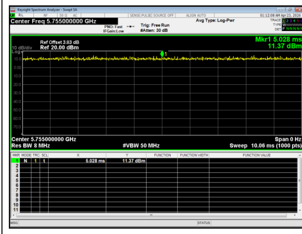
(802.11ac40) plot
