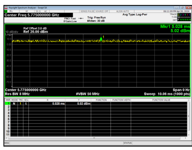
(802.11ac80) plot
