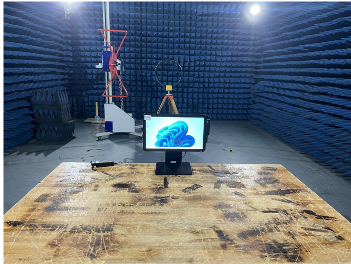
(9k-30M)
