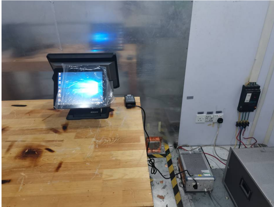
Conducted Test Setup Photograph(HK578(15 inch*10.4 inch))
