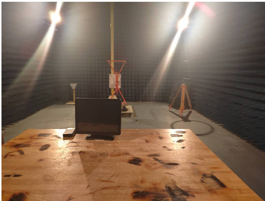
Radiated Test Setup Photograph(HK578(15 inch*15 inch))
