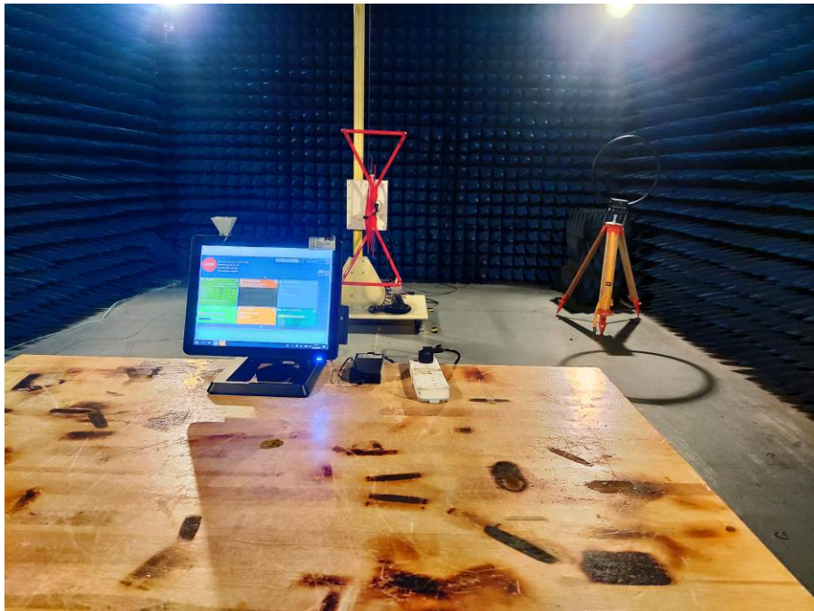
Radiated Test Setup Photograph(HK578(15 inch*10.4 inch))
